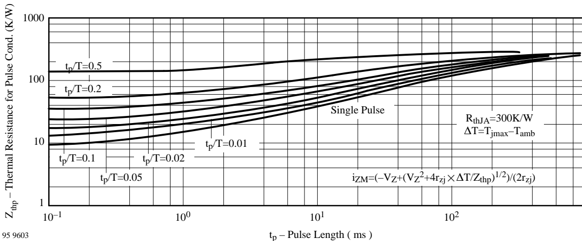
Figure 11 : Thermal Response
